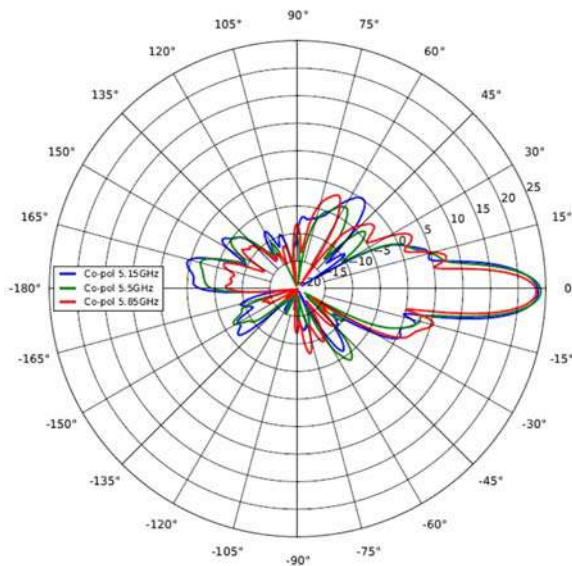
Elevation, Horizontal
