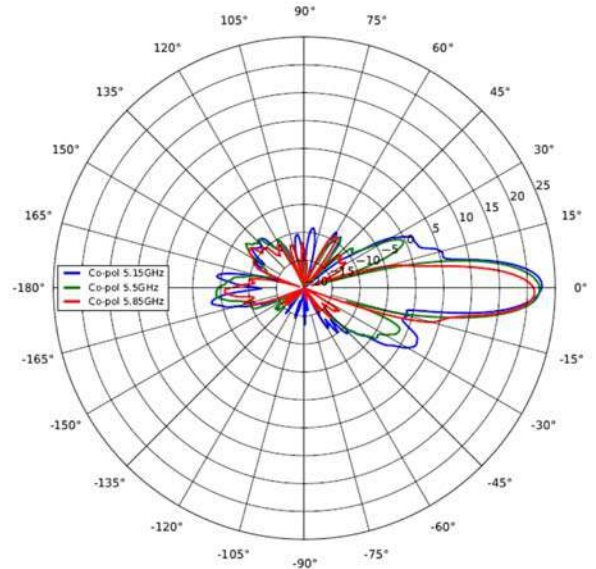
Elevation, Vertical
