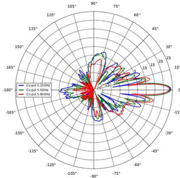
Elevation, Horizontal
